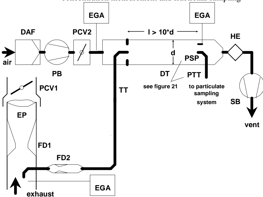
Figure 16 em with twin venturi or twin orifice, crement and fractional sampling
