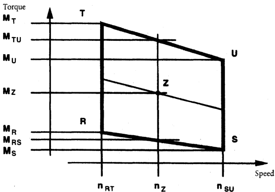
Figure 4 Interpolation of \text{NO}_x Control Point
