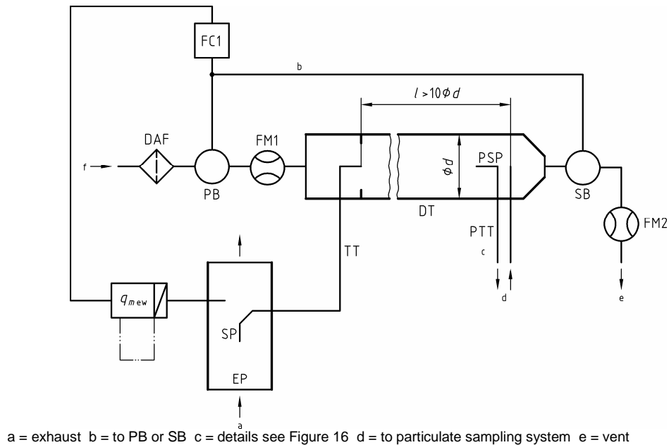
Figure 13 Scheme of partial flow dilution system (fractional sampling type)
